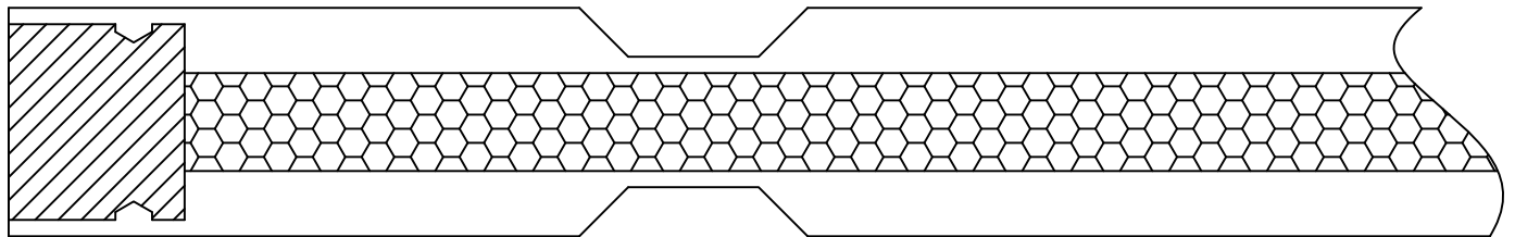
1-3/4" ENCORE - BEVEL STICKING FOAM CORE
